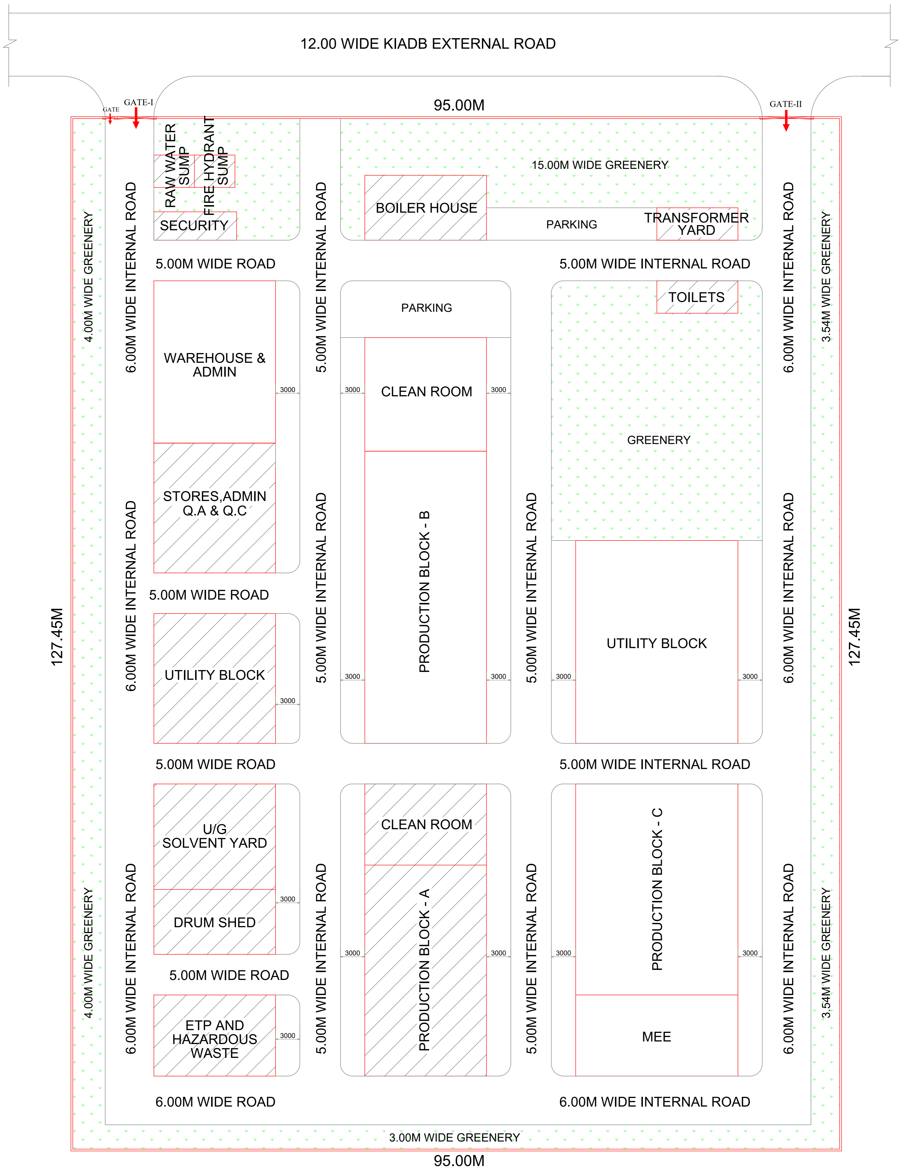
PLOT PLAN
